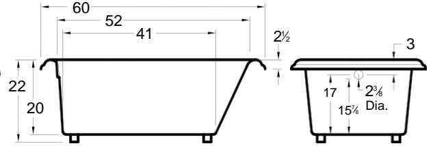
All bathtub dimensions are ± 1/2".
