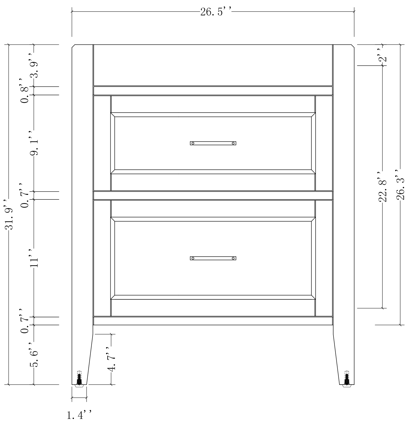
FRONT VIEW
