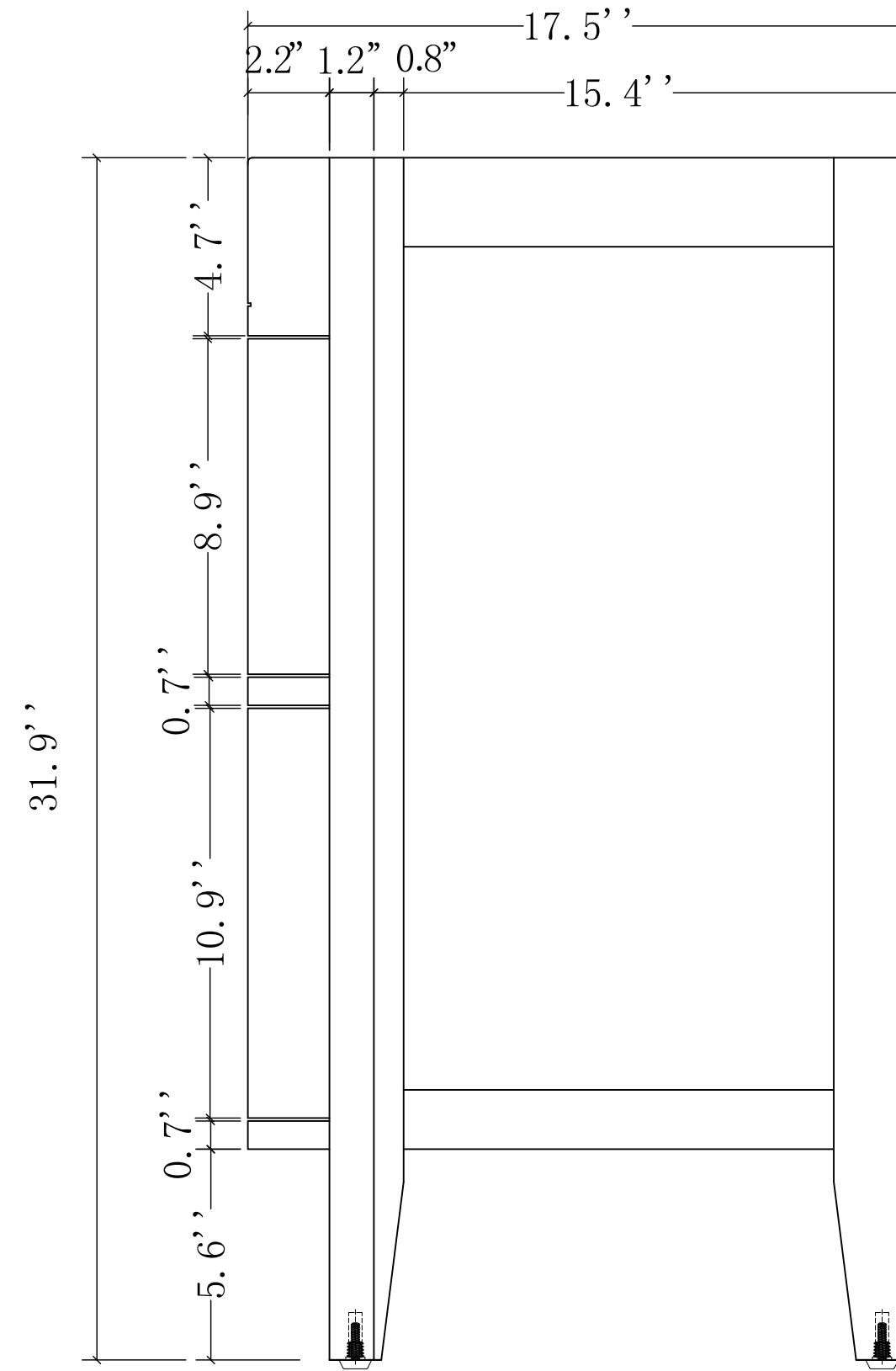
SIDE VIEW
