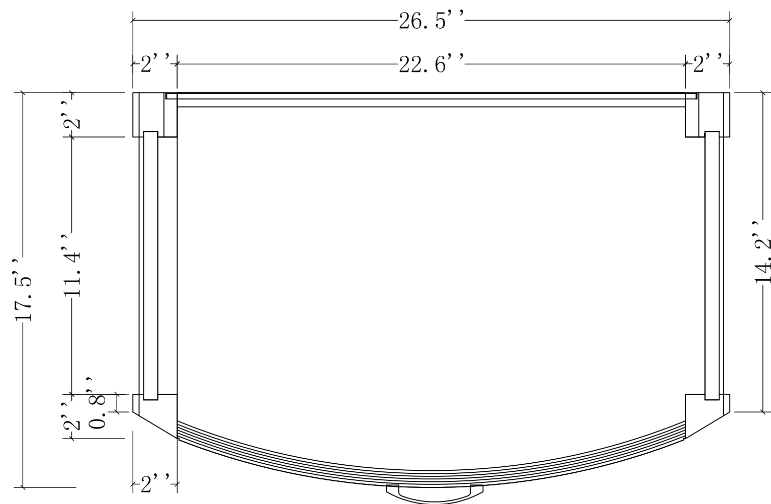
TOP VIEW
