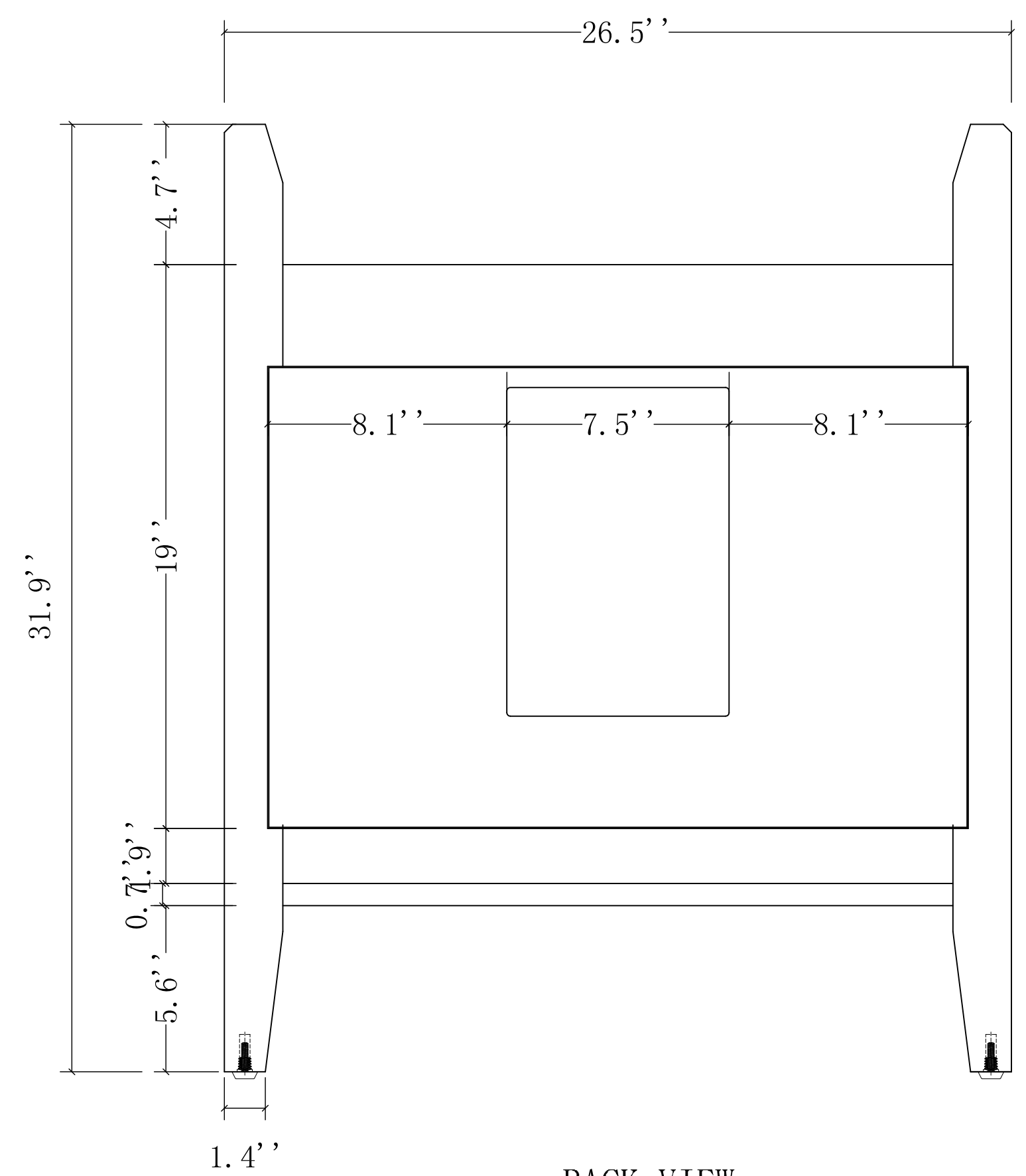
BACK VIEW
