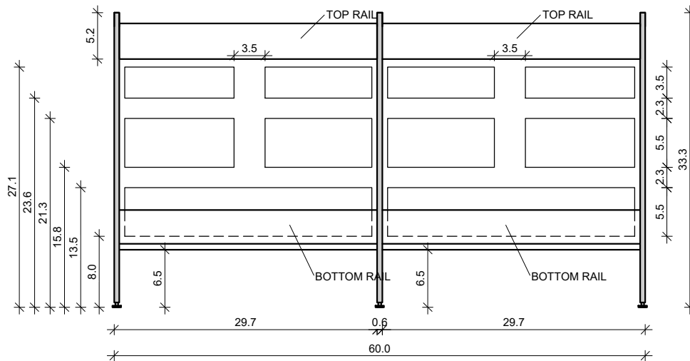
Back View
