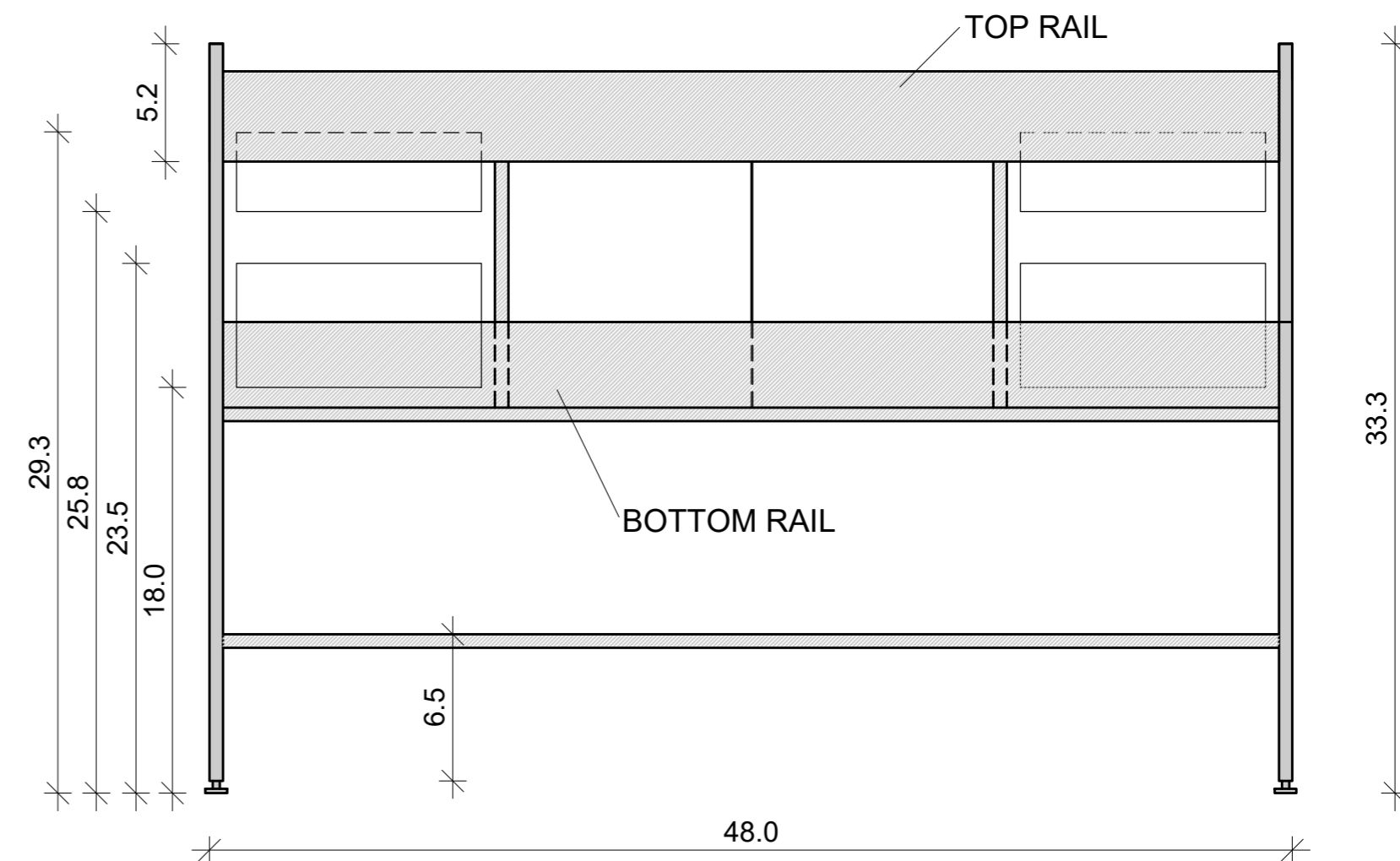
Back View
