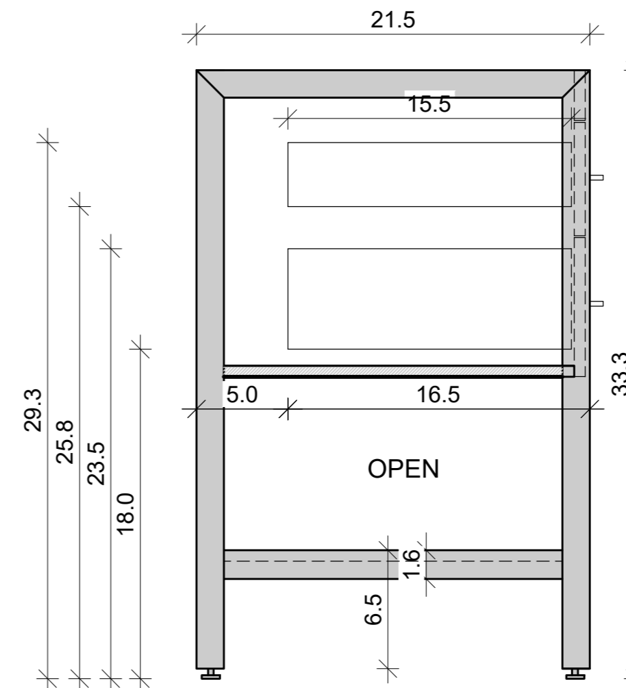
Side View
