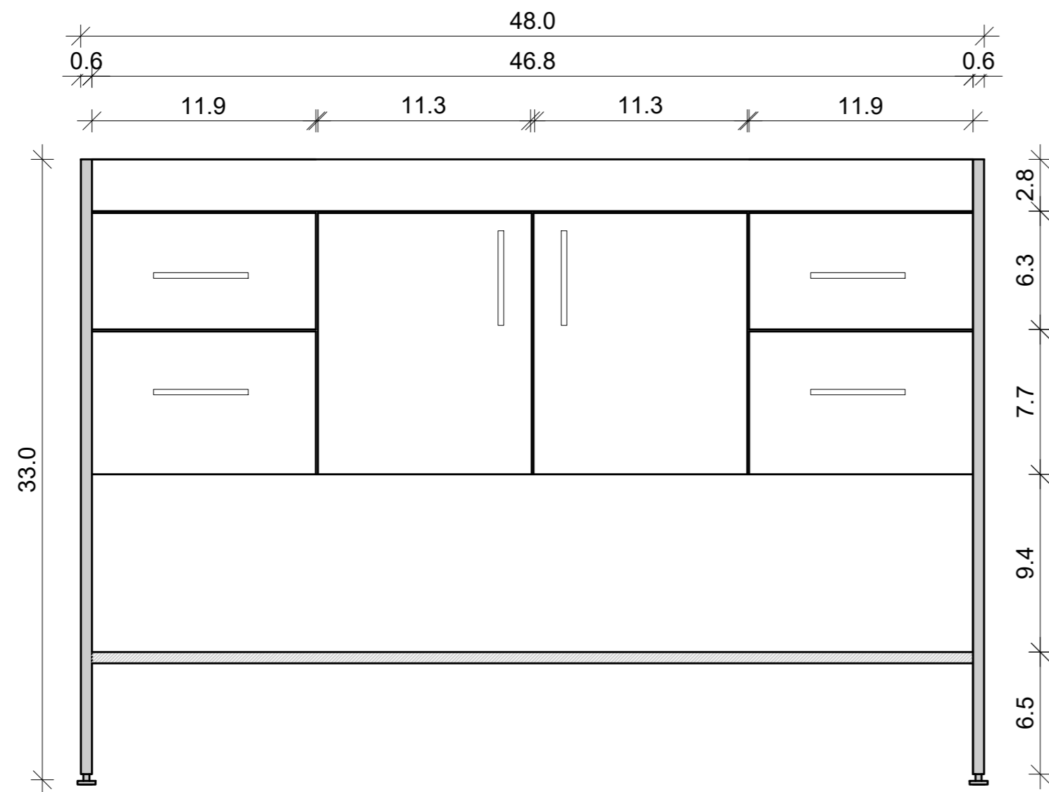
Front View
