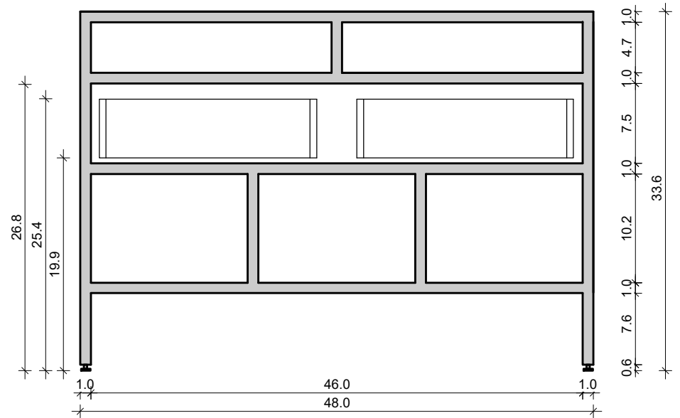
BACK VIEW
