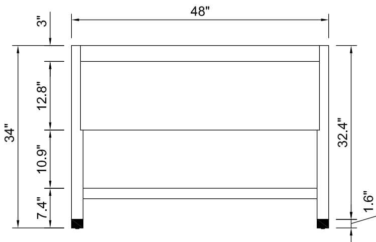
BACK VIEW
