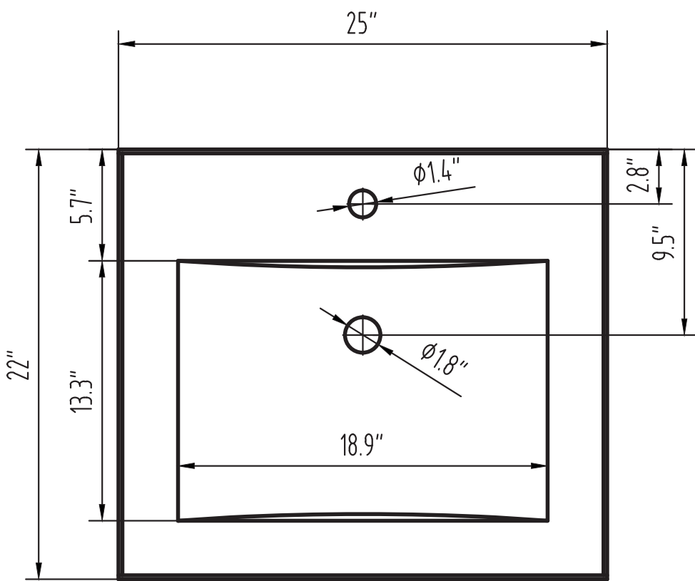
TOP VIEW
