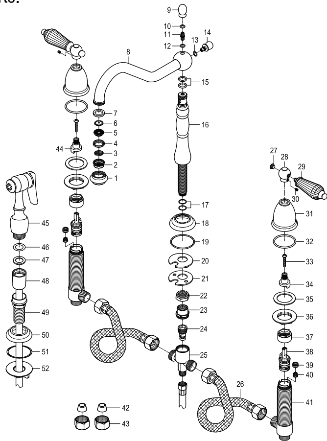
Cartridge: KBRP101C
